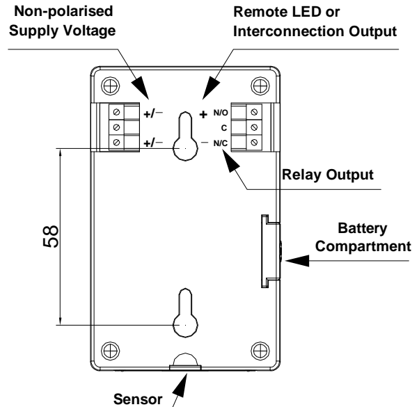
Fig. 1: 404 wiring connections
