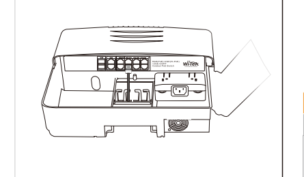
Connect Cable
