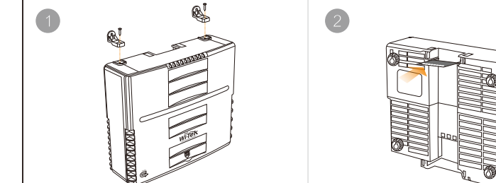
Hanging Mount
